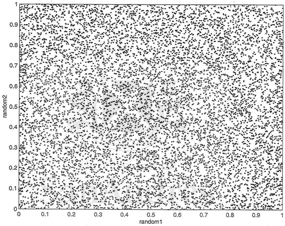
Figure 2: Distribution of 10,000 pseudo-random pairs
