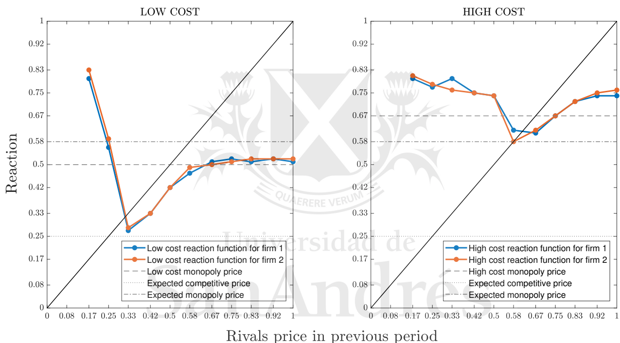
Figure 9: Reaction functions
