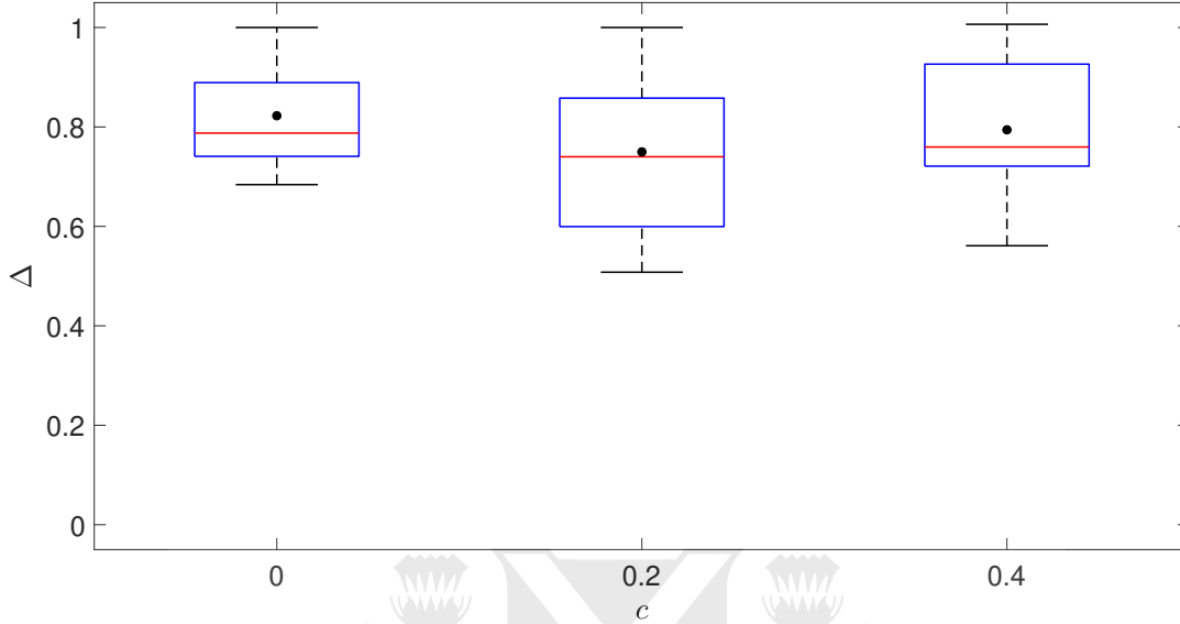
Figure 4: Normalized profits
